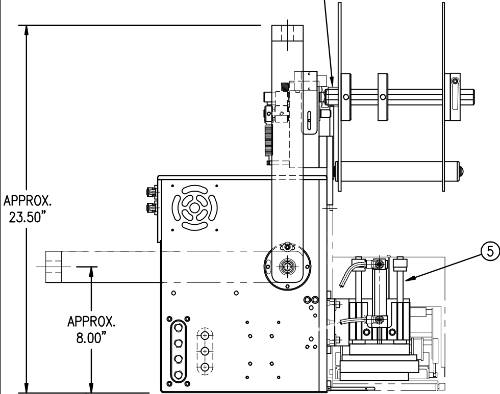
PRINT ENGINE AND CORRESPONDING WIRING HARNESS TO BE ORDERED SEPARATELY SEE CHART ON CORE UNIT DRAWING (JOB SPECIFIC)
