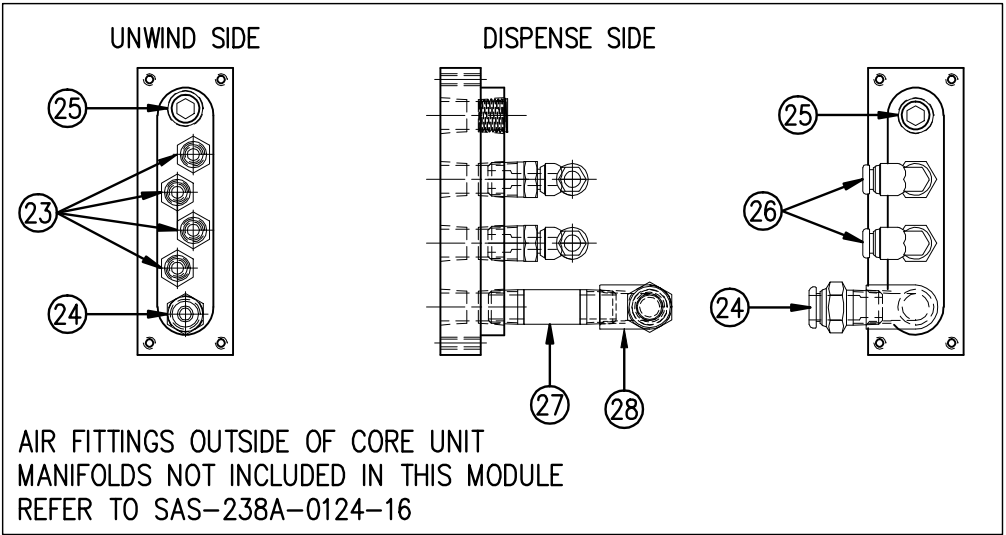
17 VALVE BANK ASS-238-0129M
