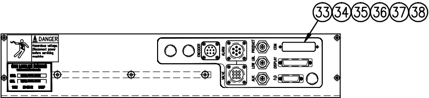
SECTION A-A CONNECTOR FACEPLATE
