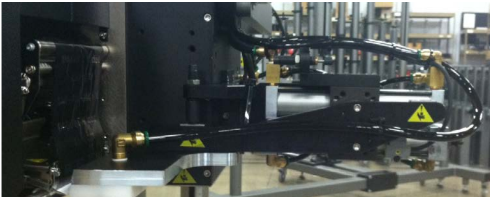
(swing tamp assembly)
