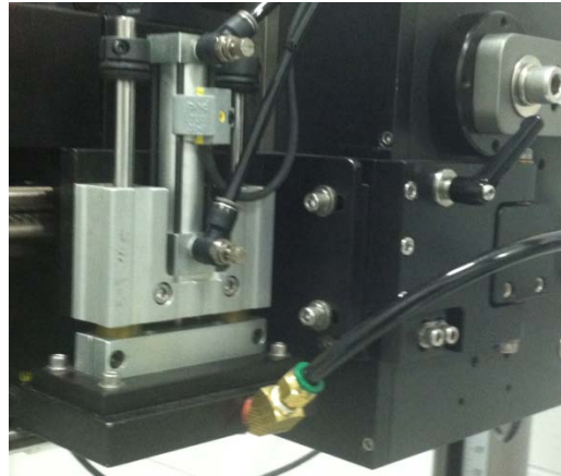
Swing-Away Tamp Assembly
