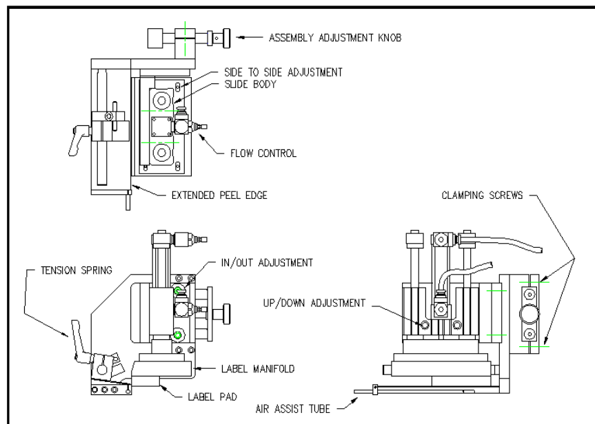
(extended peel edge assembly)
