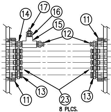
SECTION B-B TUBING & FITTINGS
