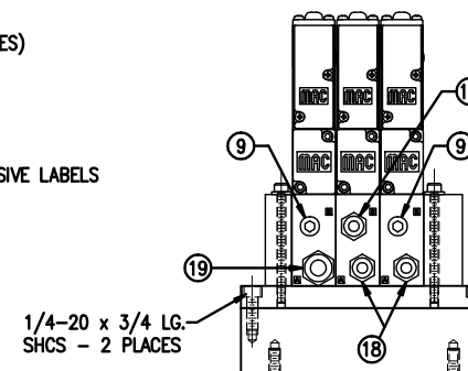
END VIEW "A" (VALVE BANK & MTG. ONLY)
