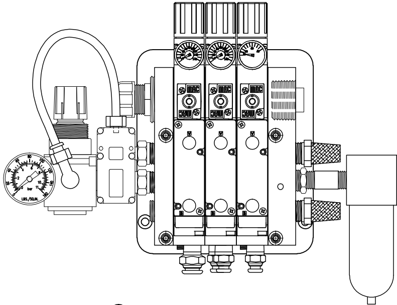
17 VALVE BANK ASS-238-0129M
