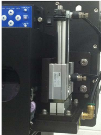
Stationary Standard Tamp Assembly
