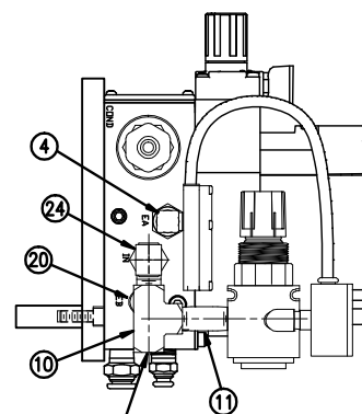
ATTACH AIR FILTER ASSEMBLY HERE FOR RH APPLICATORS
