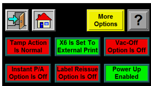
(from the standard applicator)
